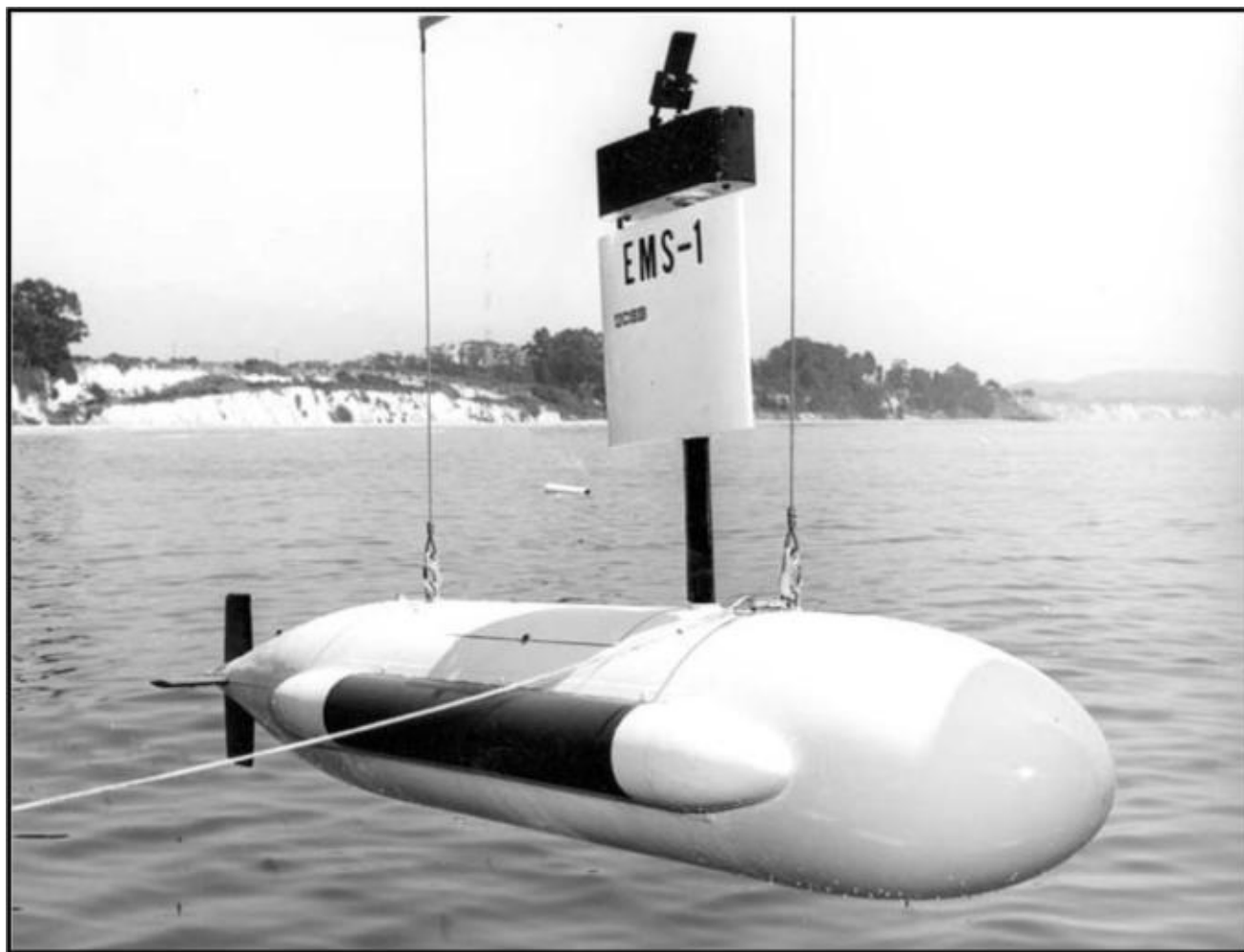
Stuart Way's electromagnetic submarine. Courtesy of the author.
