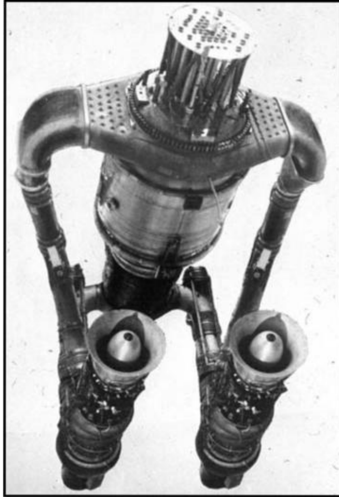
General Electric flight type XVL4-1A aircraft nuclear propulsion engine, circa 1958. Courtesy of the U. S. government.
