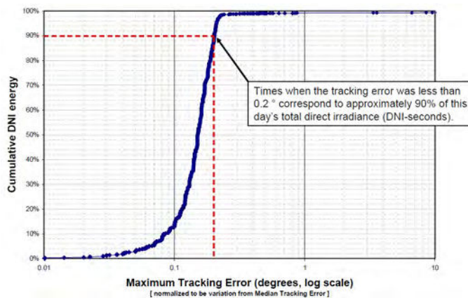
Figure 16.10 Cumulative DNI versus tracking error (Davis and Williams, 2008)
