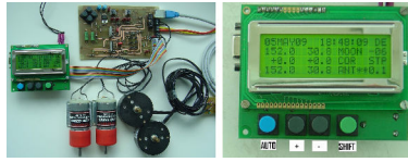
Figure 20: Parabolic dish antenna control system based on a 89C51ED2 Micro-controller (?).
