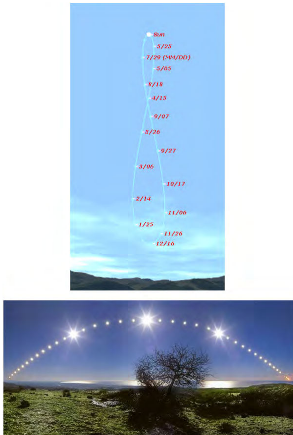
Figure 1.19 Photographic illustrations of the sun path for a single day (bottom), as well as daily photographic snapshots of the sun position taken at noon every day for a full year (top) to show the Analemma curve (Siegel, 2014).
