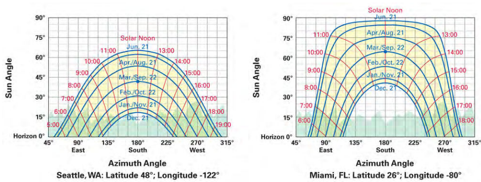
Figure 7.6 Sun part diagrams for Seattle and Miami in the USA showing vastly different solar tracking movement patterns (Homepower, 2014).
