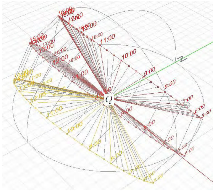
Figure 1.8 Computed sun vectors and sun path as seen by an observer at Q during winter solstice, equinox, and summer solstice (Wood, 2010).
