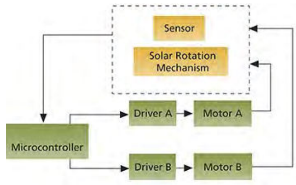
Figure 7.5 Solar tracking control architecture and block diagram (Xinhong et al. , 2007).
