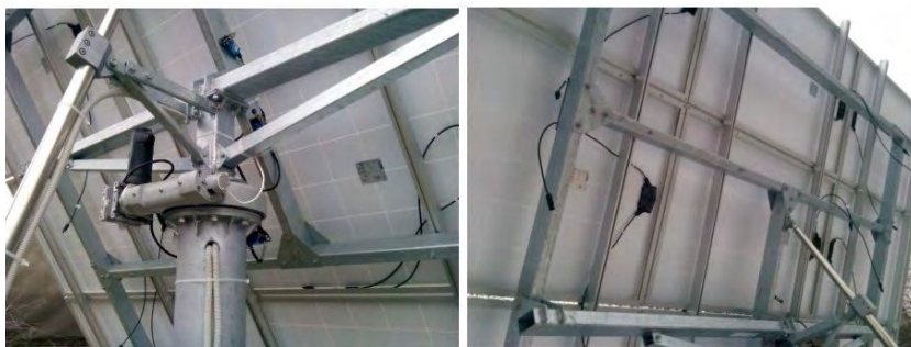
Figure 21.10 Combined linear drive and rotation drive pan-and-tilt sun tracking system to change the angle of a solar panel array (SolarTech, 2014).
