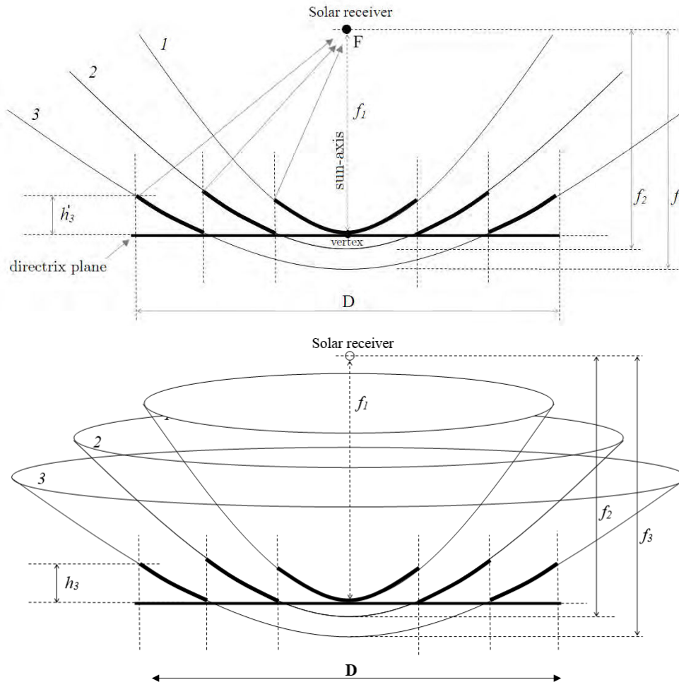
Figure 14.7 Orthographic view of a family of parabolic curves with identical parameters and focal point F , but with increasing f/D ratios, axially embedded onto the main parabolic directrix plane, serving as flat load bearing structure.
