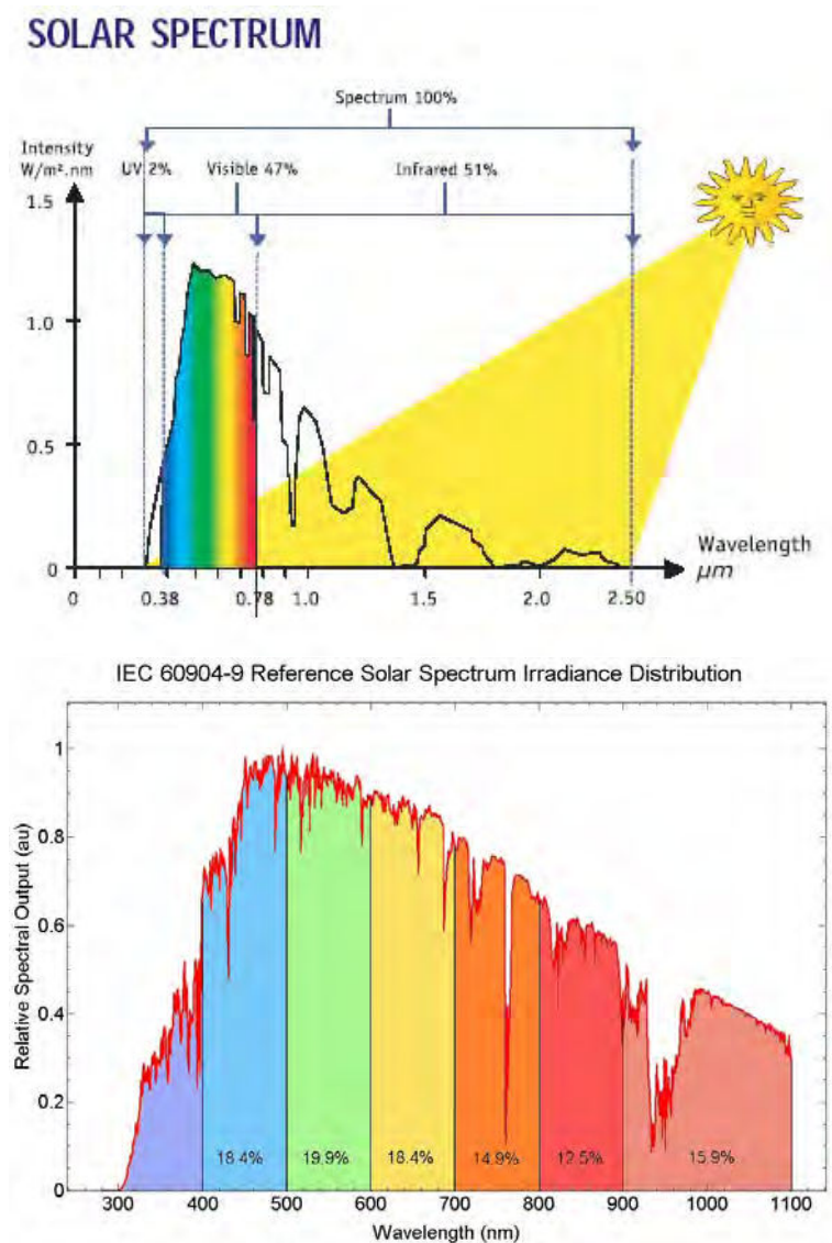
Figure 13.3 Color band spectrum for normally incident solar at sea level on a clear day (top) and solar spectrum color balance classification bands (bottom) (IEC, 2007).
