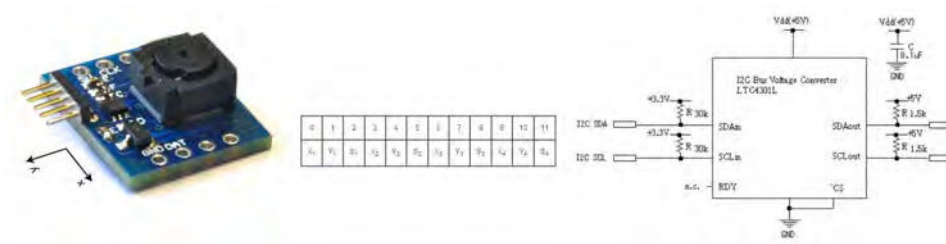
Figure 5.15 Wiimote PixArt camera with built-in multi object infrared tracking (Pixart, 2014).
