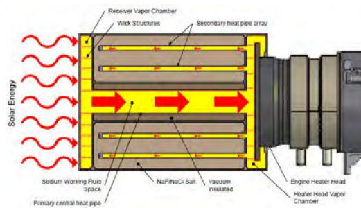
Figure 22.7 Solar receiver incorporating a salt storage device in solar receiver to counter cloud cover interruption of the PCU operation (Infina, 2012b).
