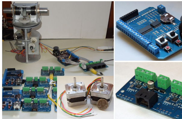
Figure 18: Arduino Sun Harvester Shield with Sun Harvester Driver Board used in sun tracker or heliostat applications with stepper motors (altitude motion and azimuthPan/Tilt) to realize a servo platform with servo dual axis control motors (?).
