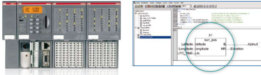
Figure 6: Scalable PLC AC500 with solar position algorithm implemented directly in the software with a high resolution ensure that the solar plant is always precisely aligned with the sun (?).
