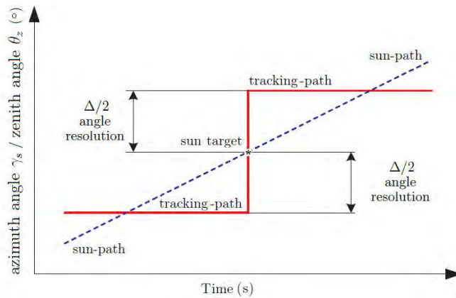
Figure 8.9 Illustration of decision logic used to control the actuator DC motor in following the sun path at tracking resolution \Delta/2 on each control axis (Prinsloo, 2014b).
