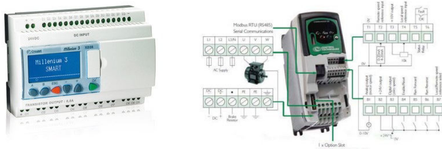
Figure 16: Crouzet Millennium PLC automatic solar tracking controller with Emerson V/F AC drive motor controller module (?)(?).
