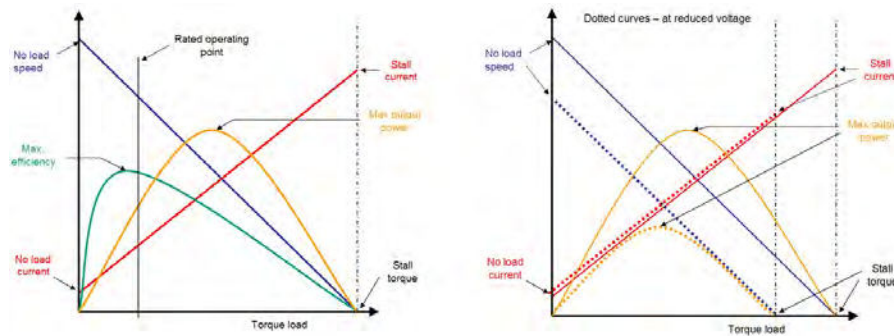
Figure 2.15 Example of motor performance curves and optimal operation points for a typical DC motor (left) and a typical DC motor running at a reduced voltage (right) (Johnson Electric, 2014).
