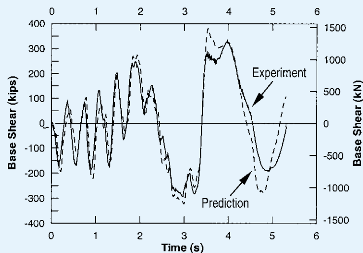
(b) Base shear force
