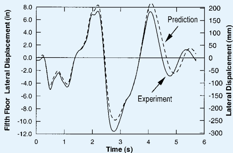
(a) Roof-level displacement
