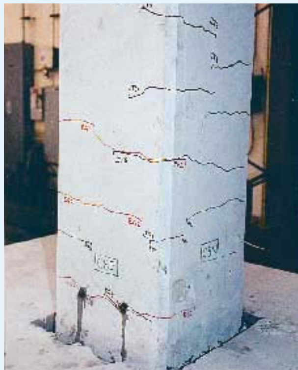
Fig. 18. Condition of various structural elements at end of testing.
