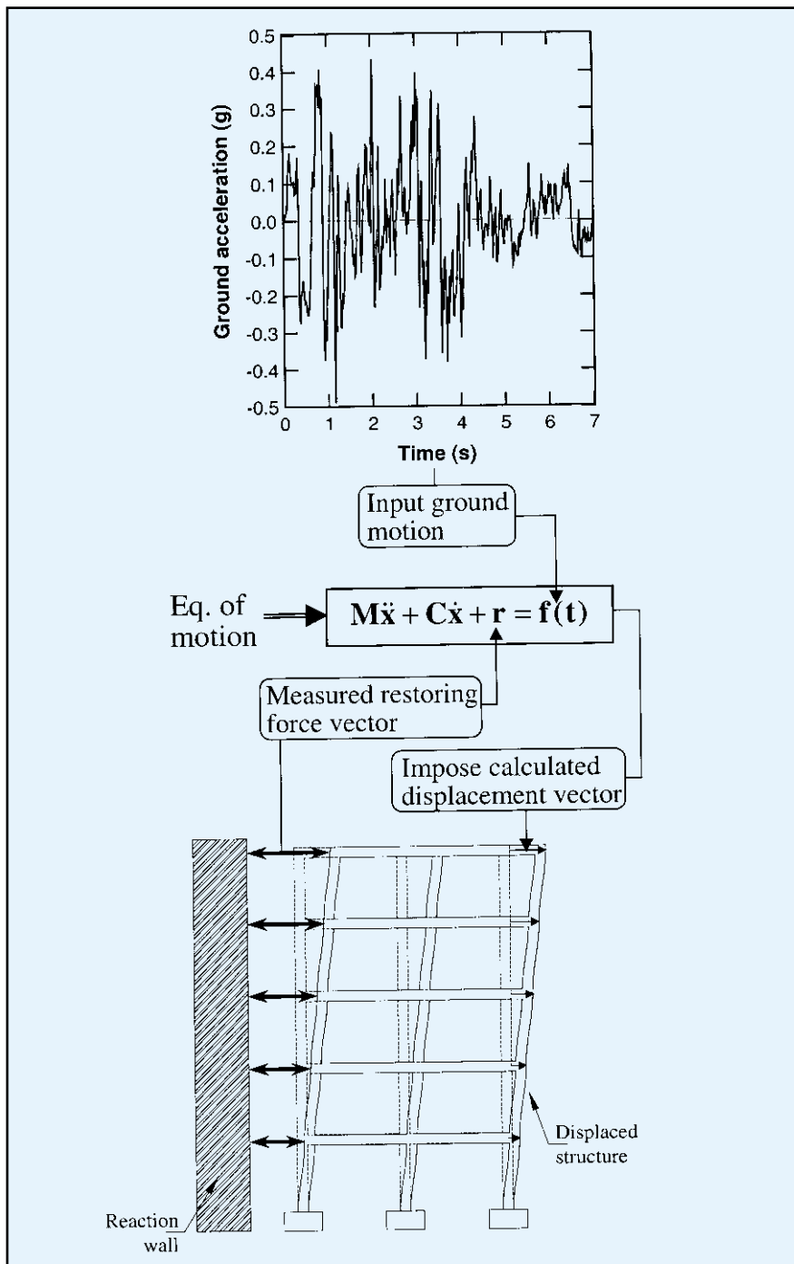
Fig. 6. Concept of pseudodynamic testing.
