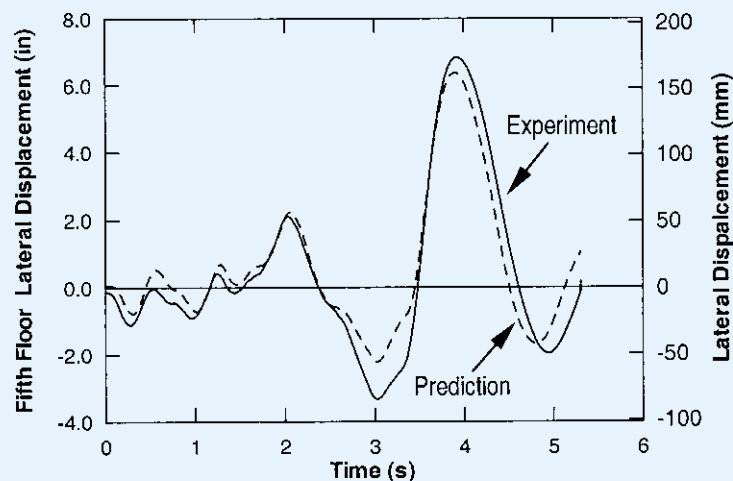
(a) Roof-level displacement
