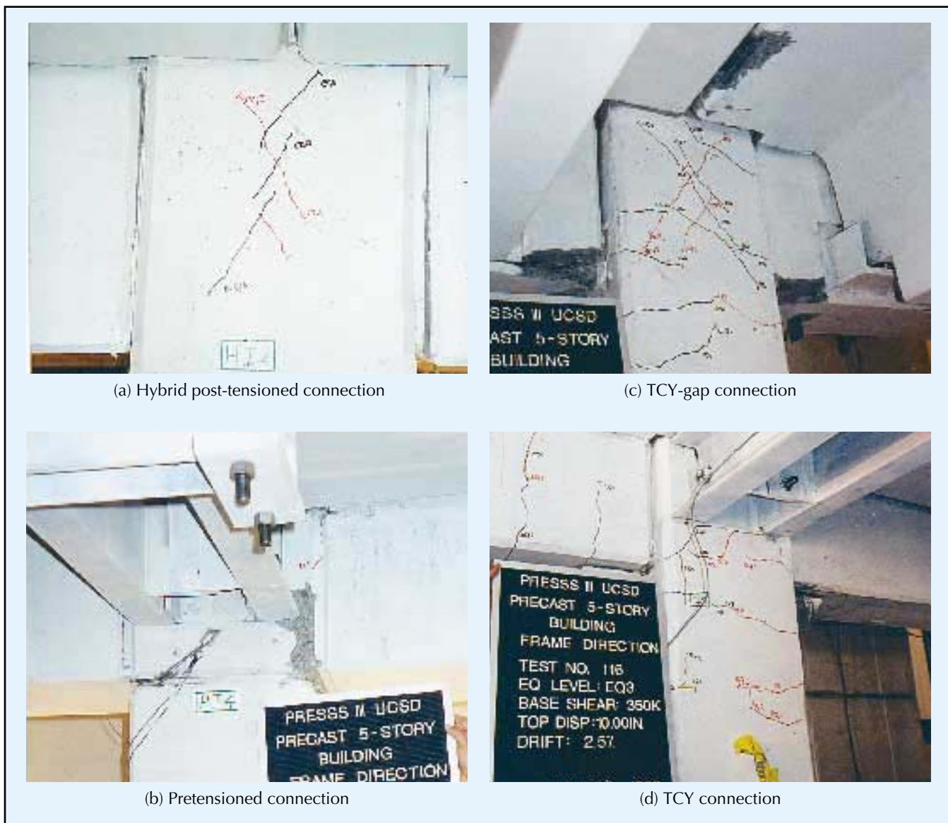
Fig. 16. Condition of frame connections after design level of response.
