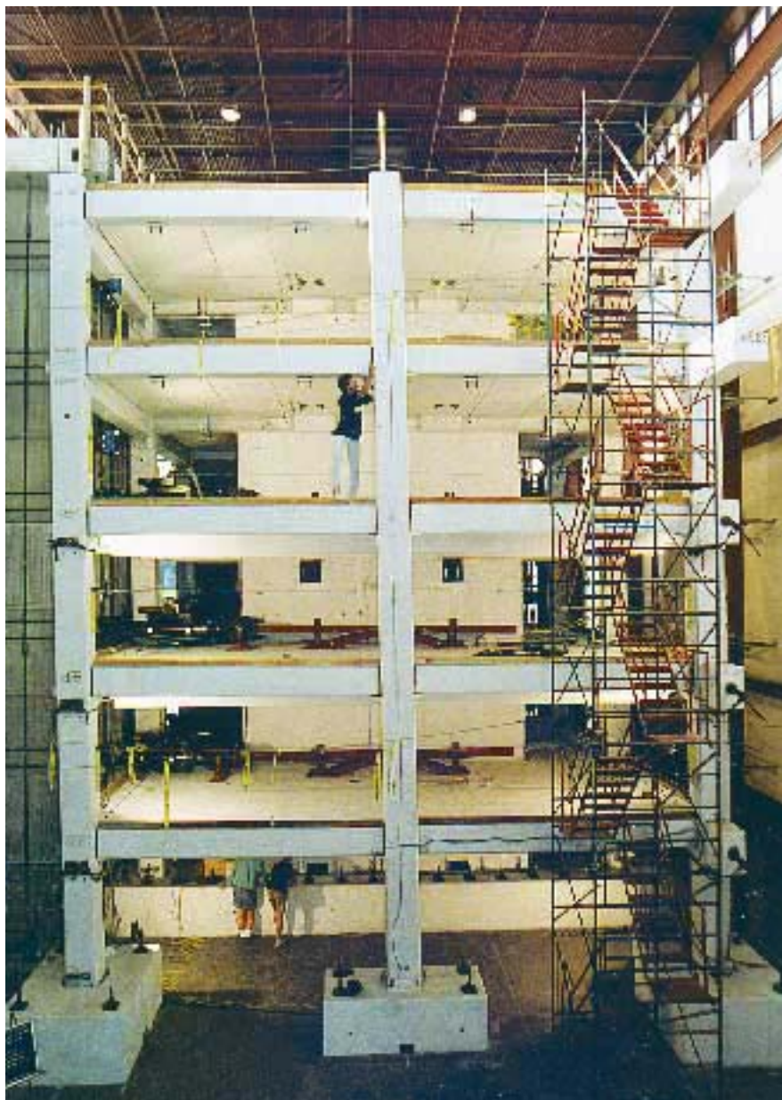
Fig. 7. Overall view of five-story building under test.
