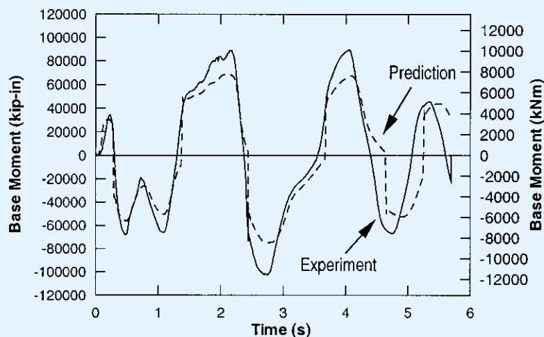
(c) Base moment
