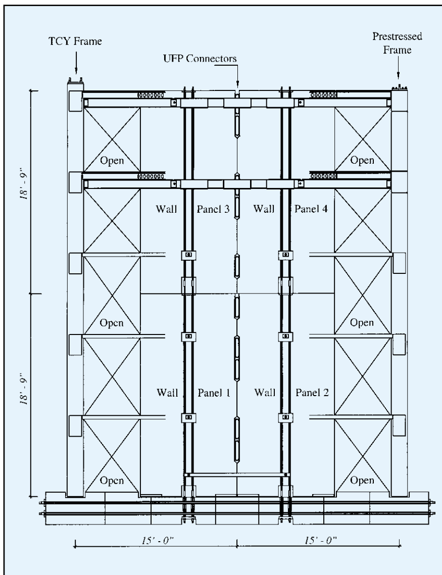
Fig. 3. Jointed structural wall elevation.
