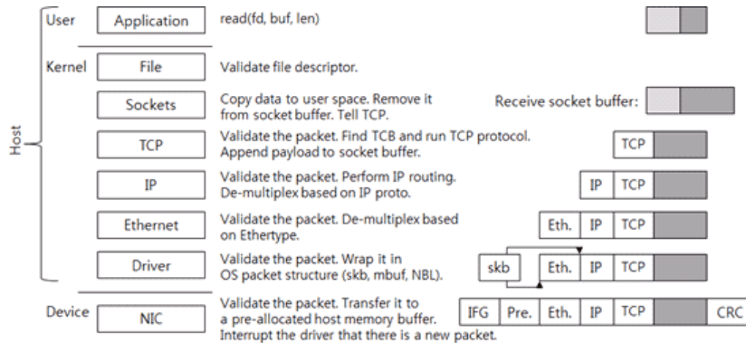
Figure 3: Operation Process by Each Layer of TCP/IP Network Stack for Handling Data Received.
