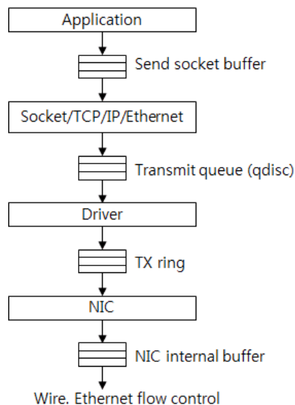
Figure 10: Buffers Related to Packet Transmission.
