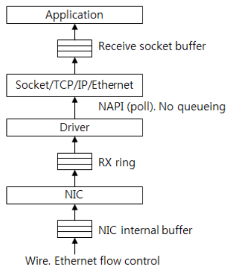
Figure 11: Buffers Related to Packet Receiving.
