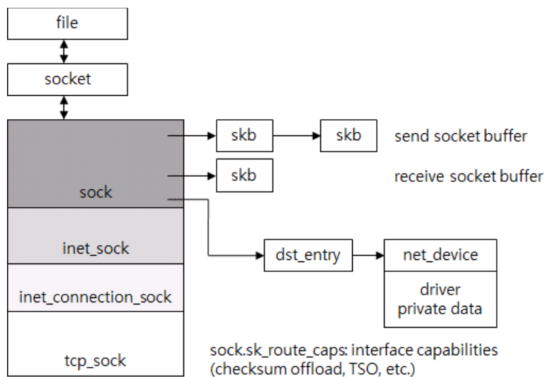
Figure 7: TCP Connection Structure.
