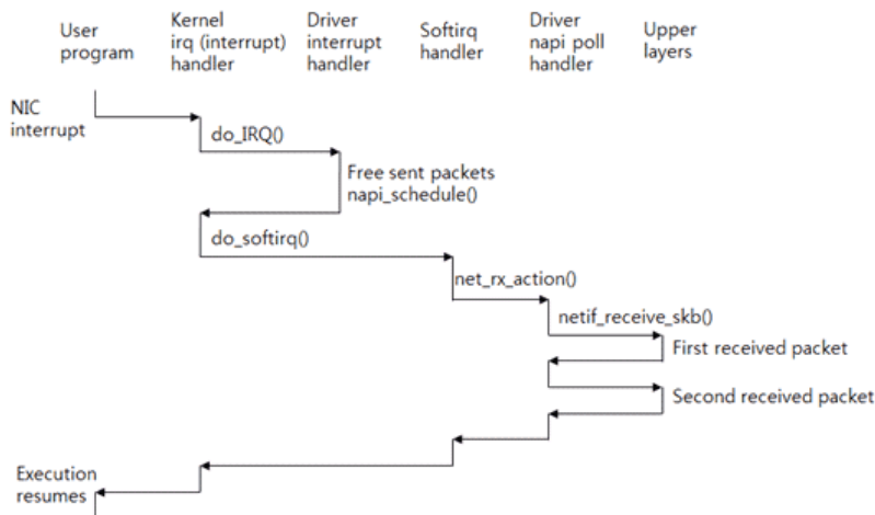
Figure 5: Processing Interrupt, softirq, and Received Packet.
