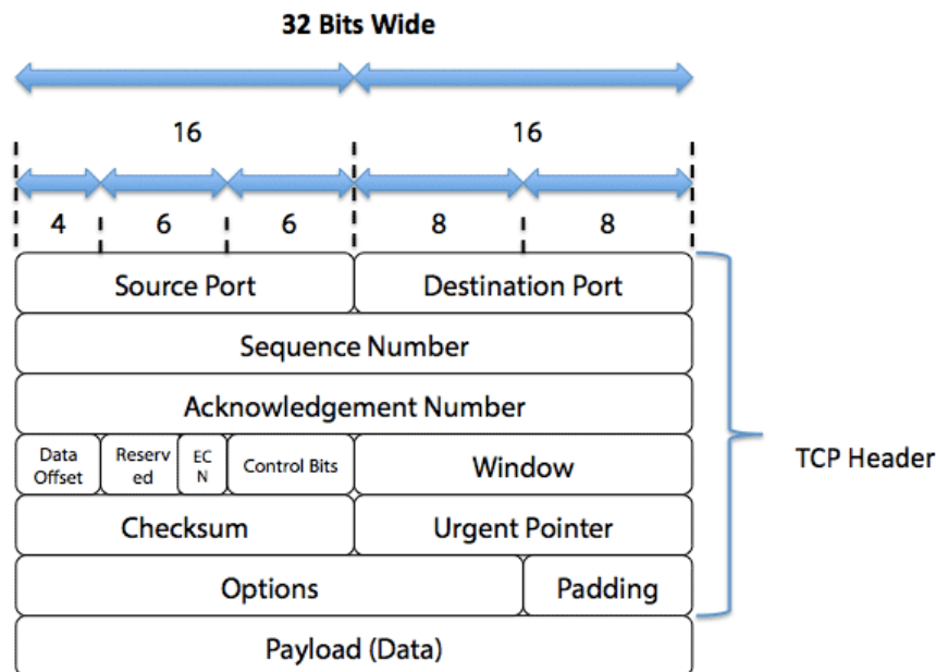
Figure 2: TCP Frame Structure (source).
