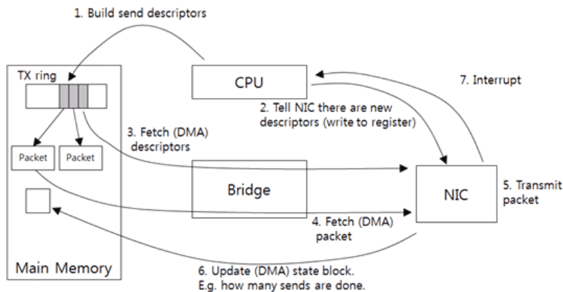
Figure 8: Driver-NIC Communication: How to Transmit Packet.
