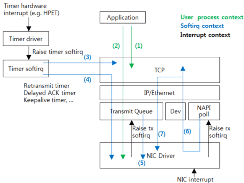
Figure 4: Control Flow in the Stack.
