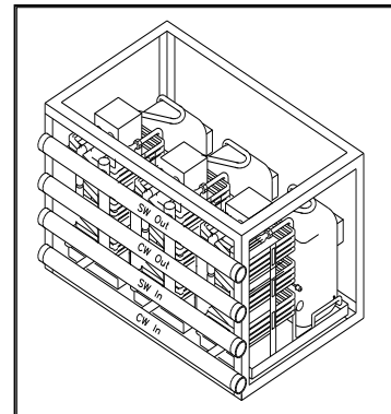
Typical framed chiller with headers
