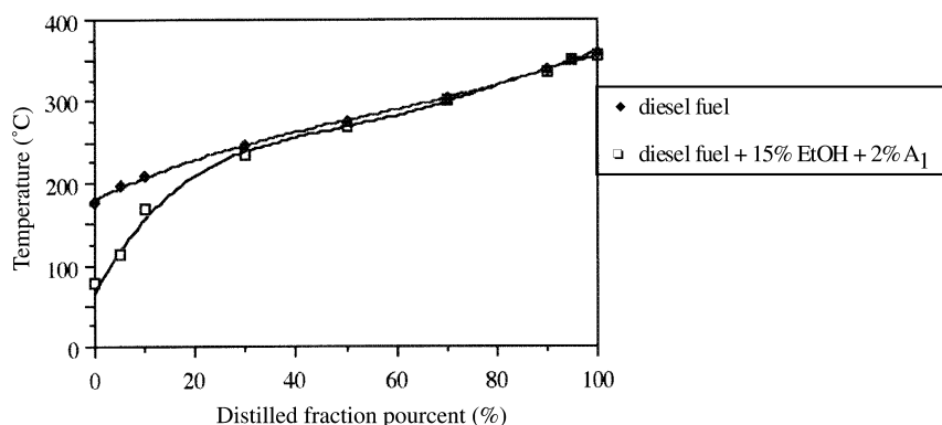
Fig. 4. Distillation curves.
