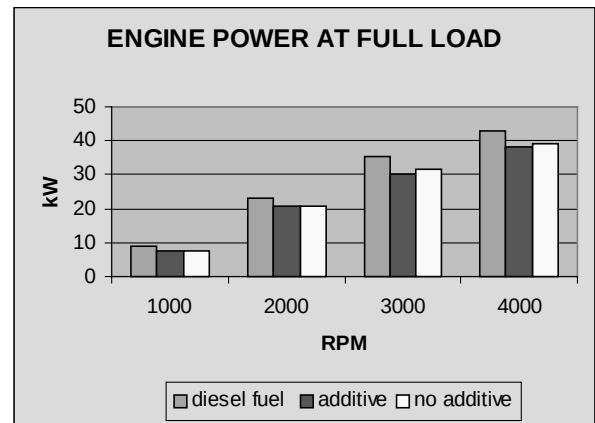
Fig. 10. Power measured on IDI Renault engine.
