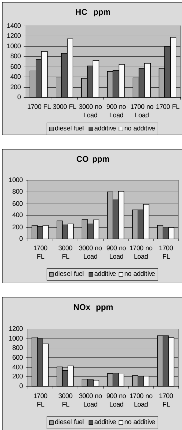
Fig. 7. Composition of exhaust fumes in a DI HATZ engine.
