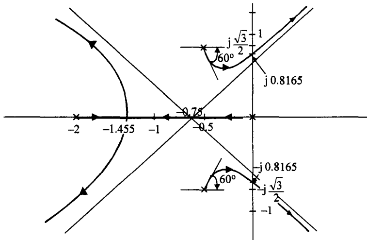
Fig. 5.14 (c) Complete root locus sketch for G(s)H(s) = \frac{K}{s(s+2)(s^2+s+1)}
