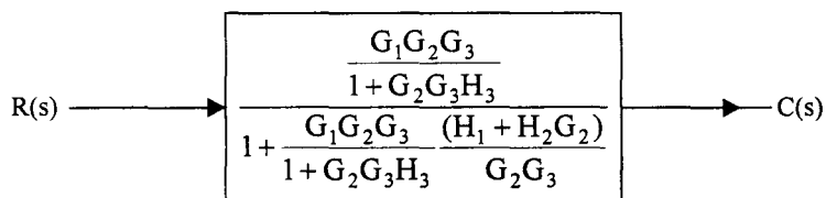
Fig. 2.34 (e) Final step in the block diagram reduction
