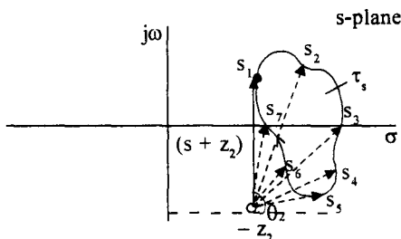
Fig. 7.3 (b) Angle contributed by (s + z_2) to F(s)
